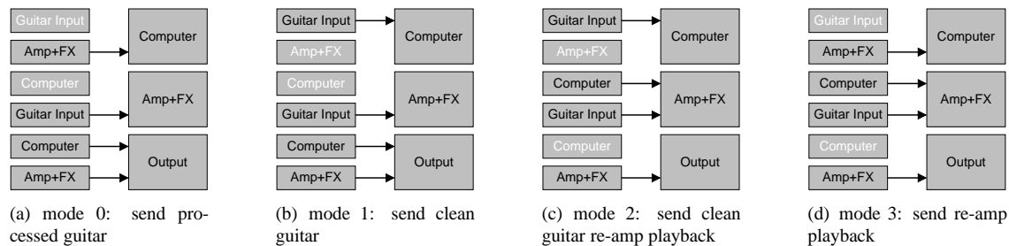
Figure 1: Different signal routing options
